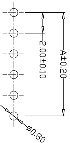
PCB LAYOUT
