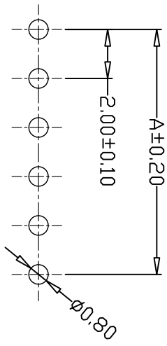
PCB LAYOUT
