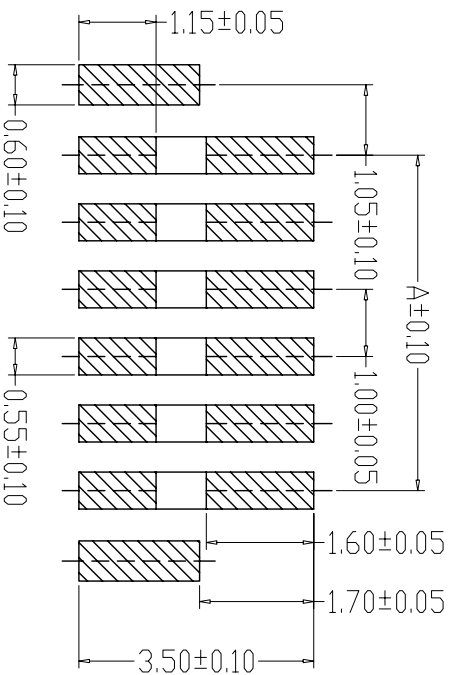
PCB LAYOUT A
